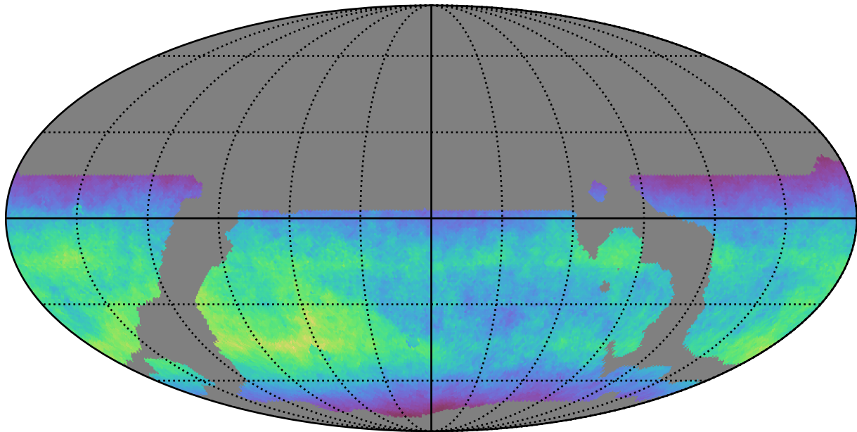
weather_cloudso6v3.4_10yrs WFD i band: Normalized Teff
