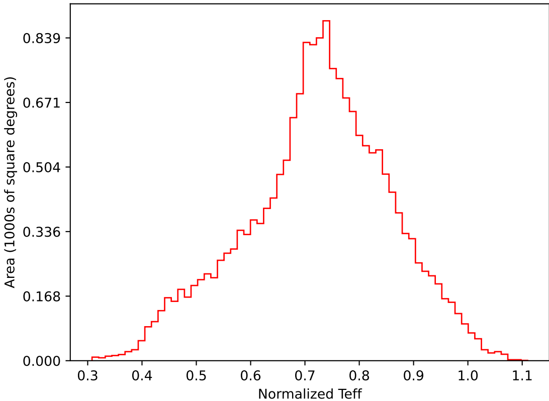
weather_cloudso6v3.4_10yrs WFD i band: Normalized Teff
