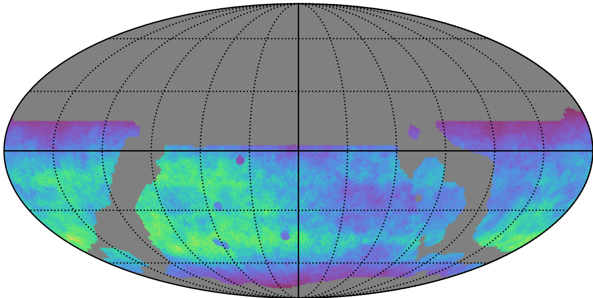
weather_cloudso6v3.4_10yrs WFD g band: Normalized Teff
