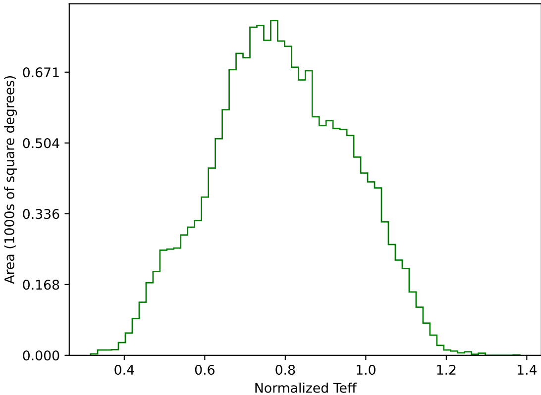
weather_cloudso6v3.4_10yrs WFD g band: Normalized Teff
