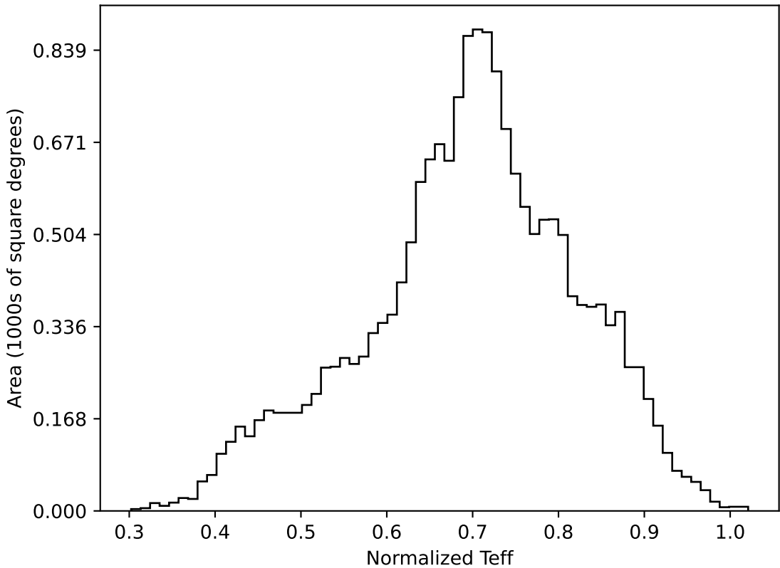
weather_cloudso6v3.4_10yrs WFD all bands: Normalized Teff
