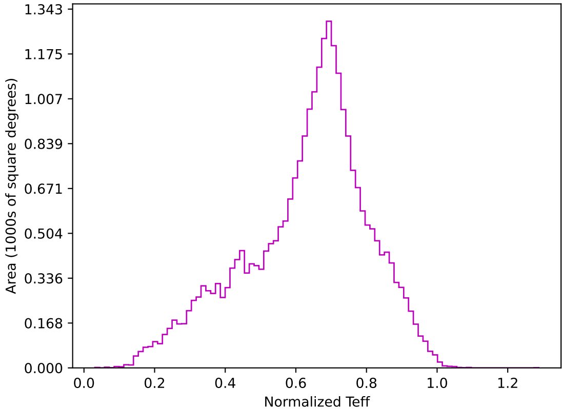
weather_cloudso6v3.4_10yrs All sky z band: Normalized Teff
