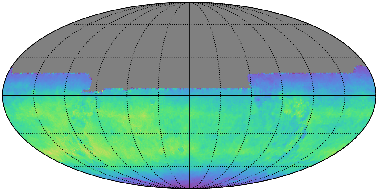
weather_cloudso6v3.4_10yrs All sky y band: Normalized Teff
