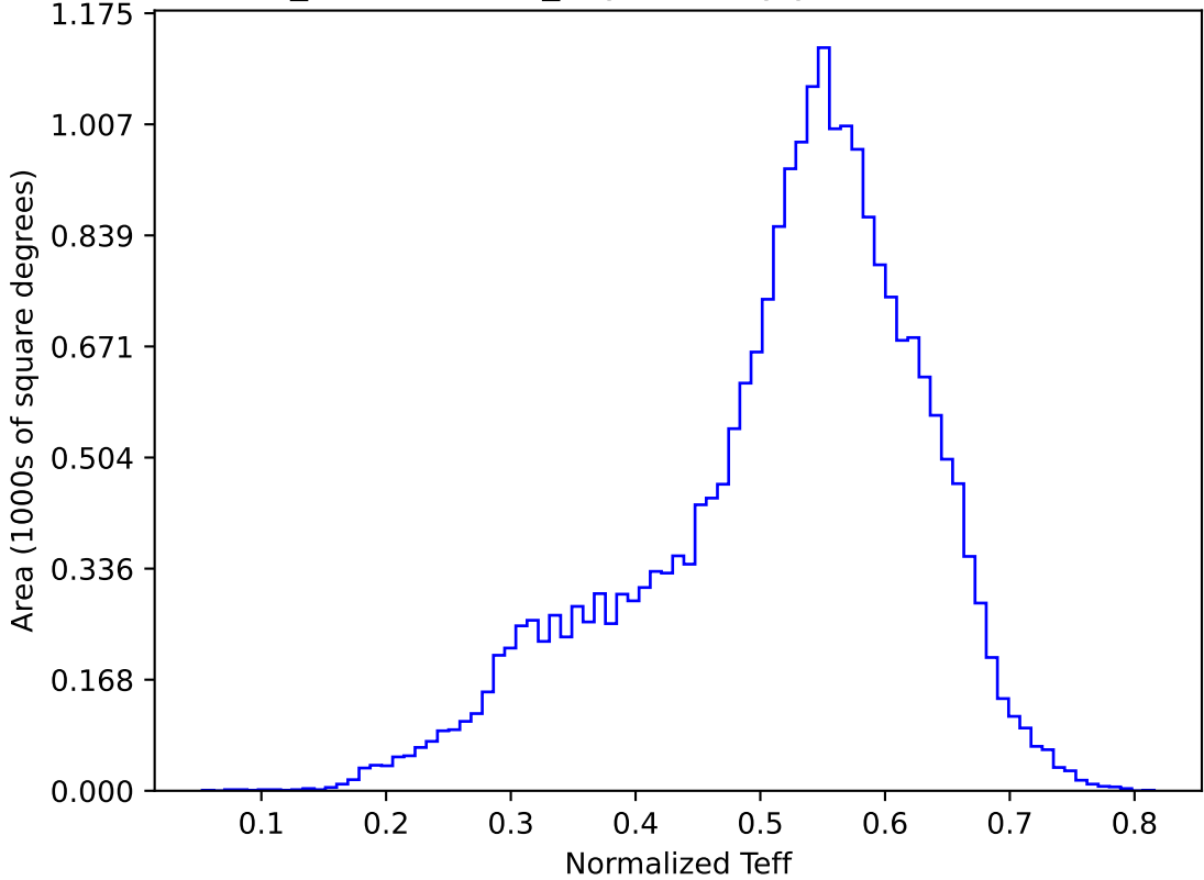
weather_cloudso6v3.4_10yrs All sky y band: Normalized Teff
