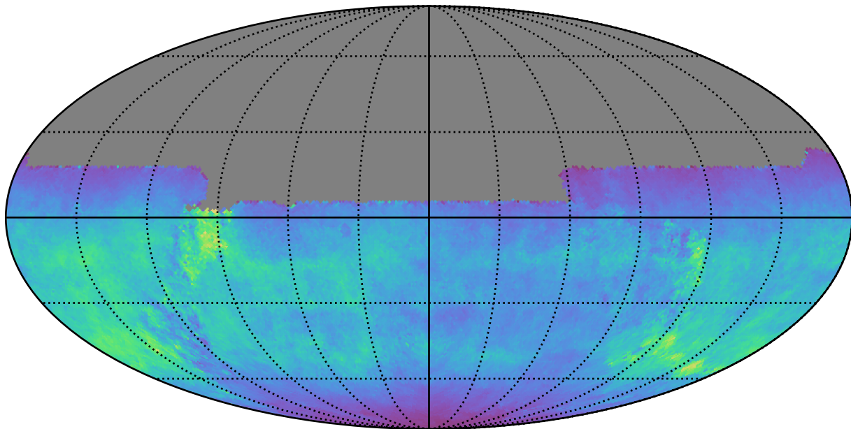
weather_cloudso6v3.4_10yrs All sky u band: Normalized Teff
