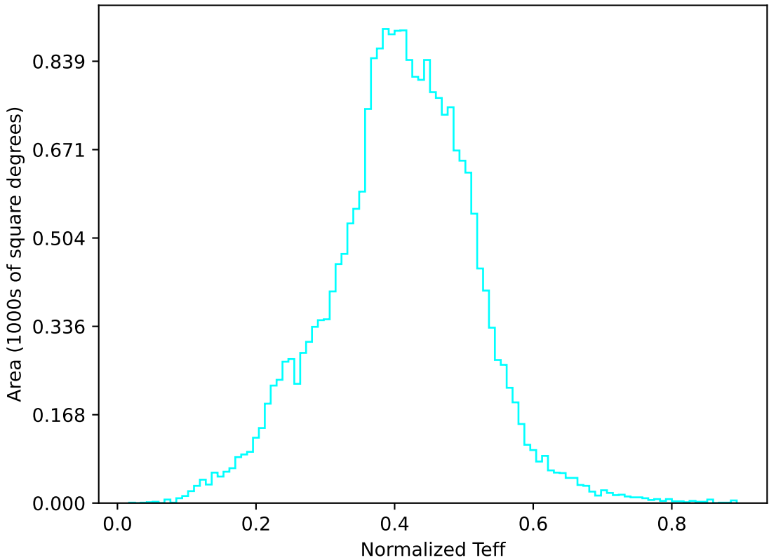
weather_cloudso6v3.4_10yrs All sky u band: Normalized Teff
