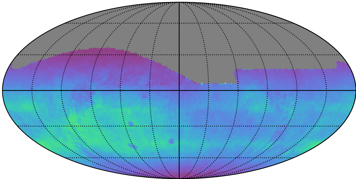
weather_cloudso6v3.4_10yrs All sky r band: Normalized Teff
