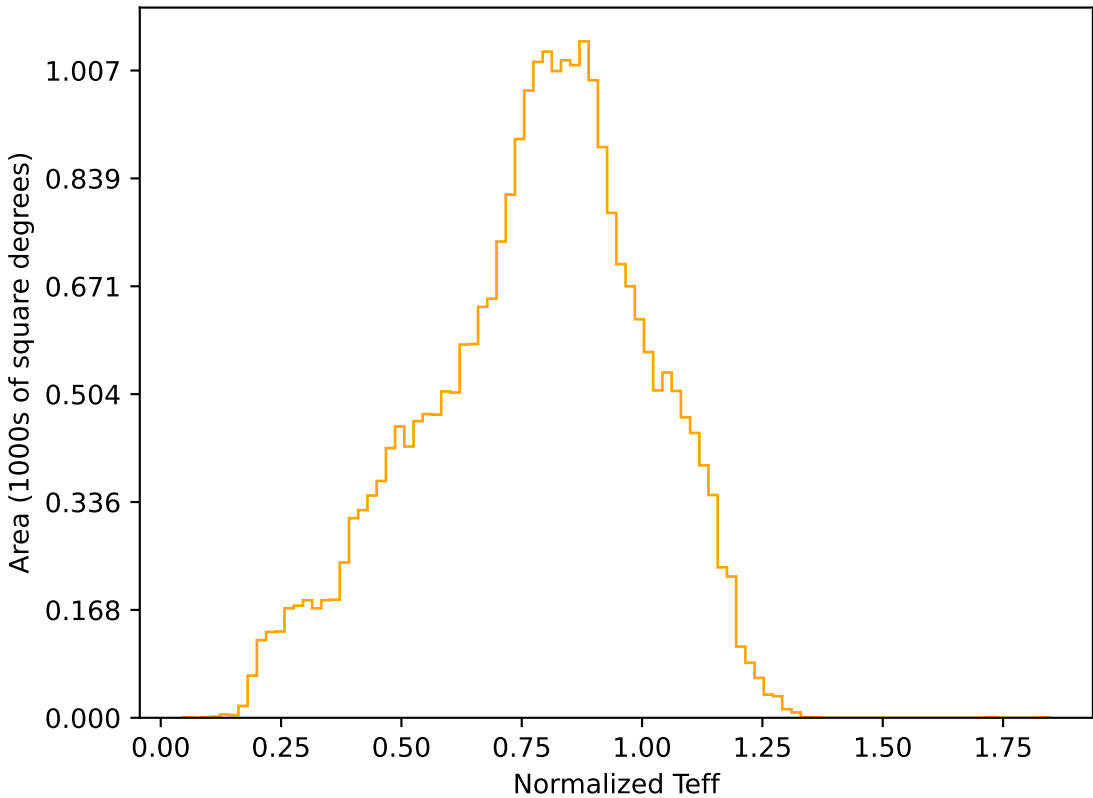
weather_cloudso6v3.4_10yrs All sky r band: Normalized Teff
