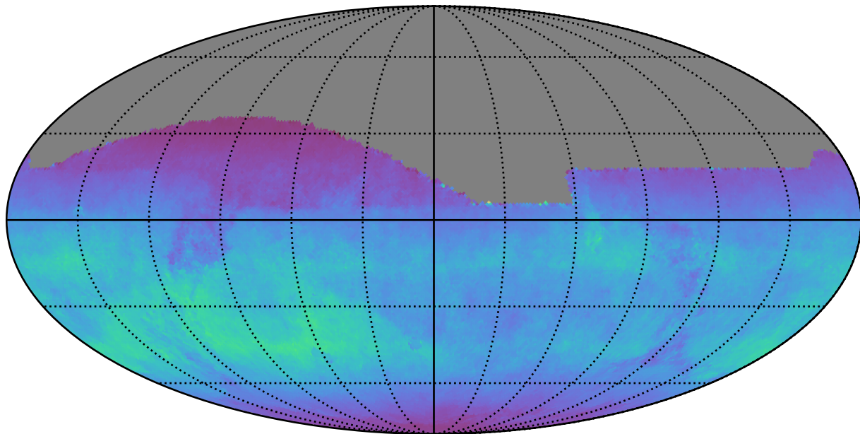
weather_cloudso6v3.4_10yrs All sky i band: Normalized Teff
