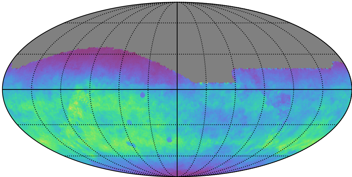
weather_cloudso6v3.4_10yrs All sky g band: Normalized Teff
