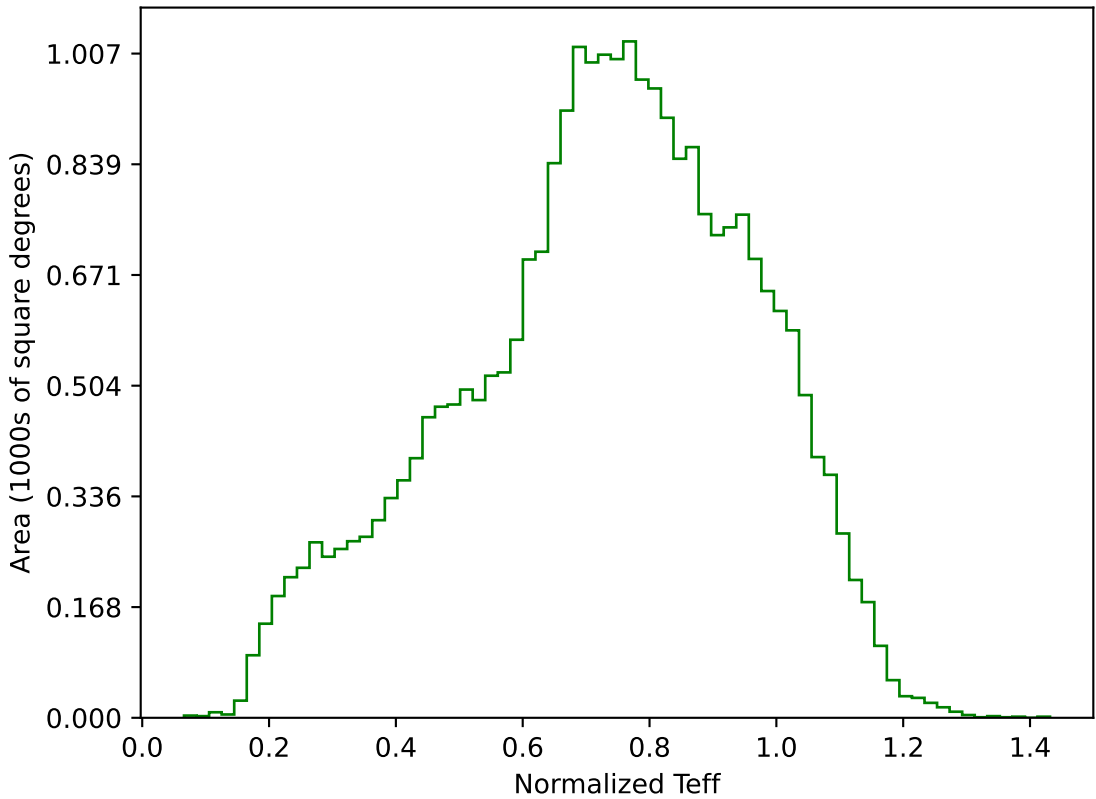
weather_cloudso6v3.4_10yrs All sky g band: Normalized Teff
