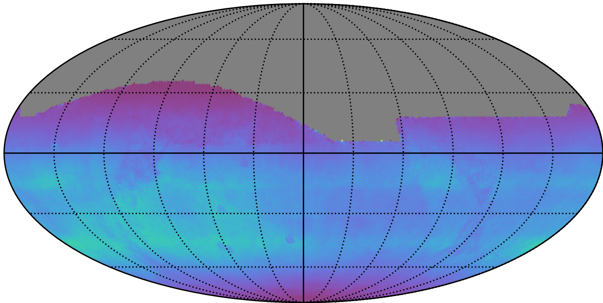
weather_cloudso6v3.4_10yrs All sky all bands: Normalized Teff
