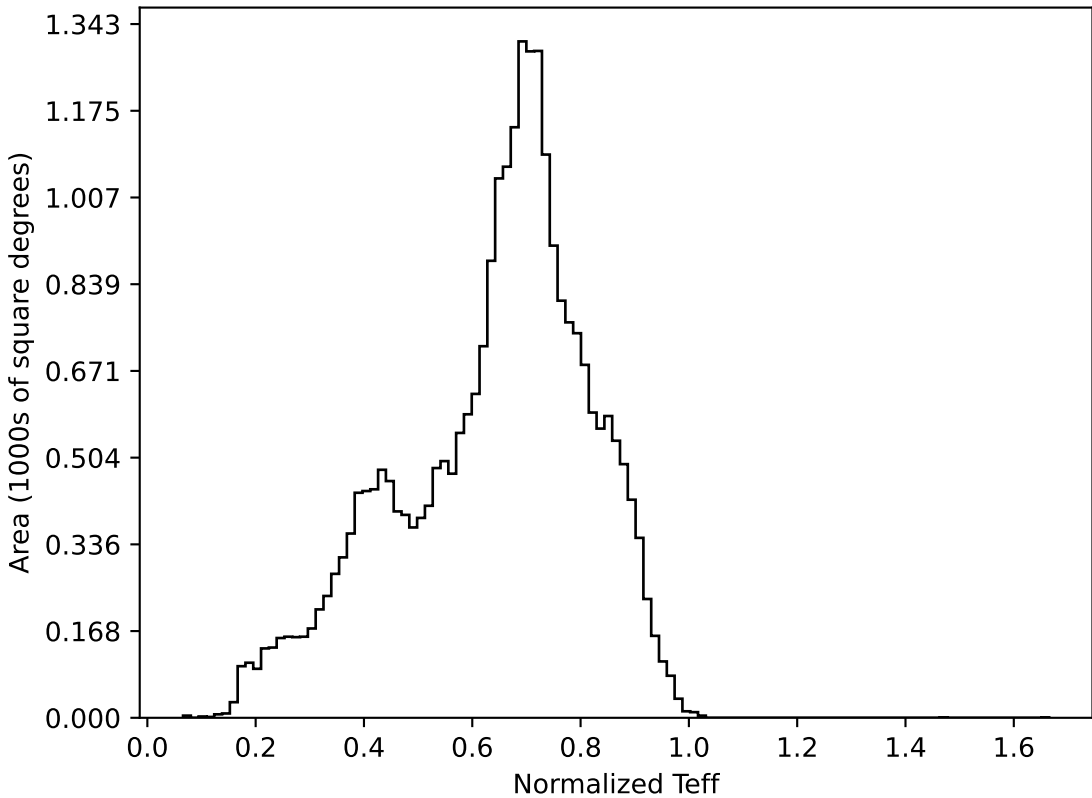
weather_cloudso6v3.4_10yrs All sky all bands: Normalized Teff
