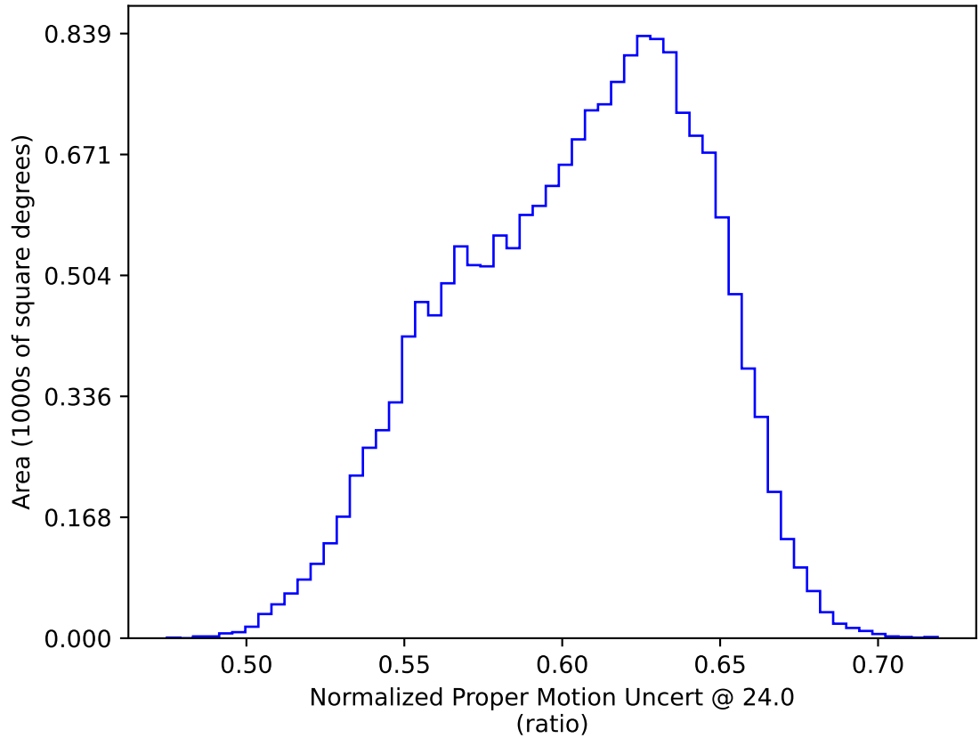
weather_cloudso6v3.4_10yrs WFD: Normalized Proper Motion Uncert @ 24.0
