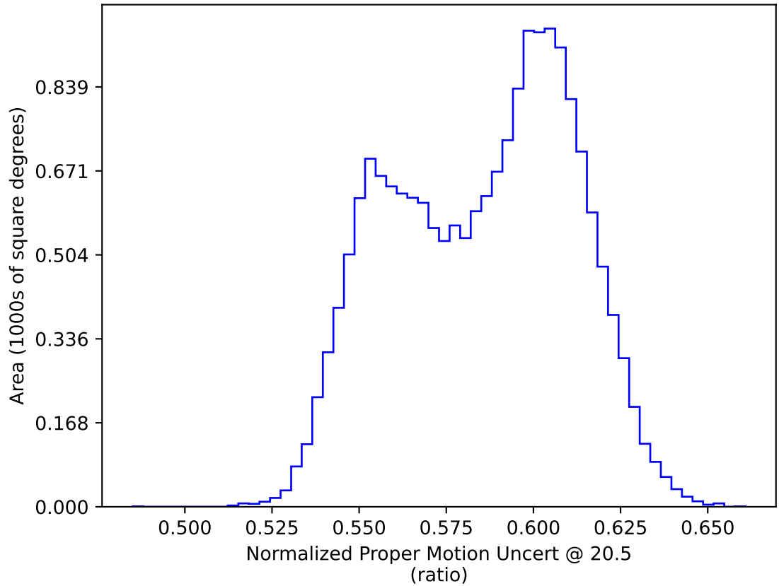
weather_cloudso6v3.4_10yrs WFD: Normalized Proper Motion Uncert @ 20.5
