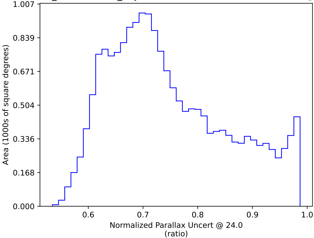
weather_cloudso6v3.4_10yrs WFD: Normalized Parallax Uncert @ 24.0
