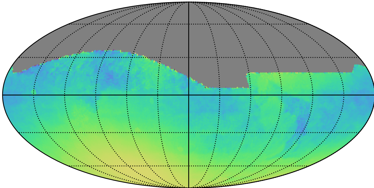
weather_cloudso6v3.4_10yrs All sky: Normalized Parallax Uncert @ 24.0
