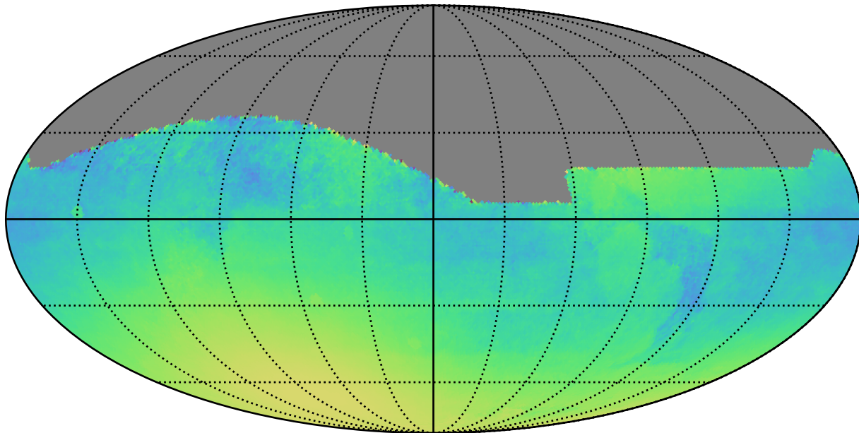
weather_cloudso6v3.4_10yrs All sky: Normalized Parallax Uncert @ 22.4
