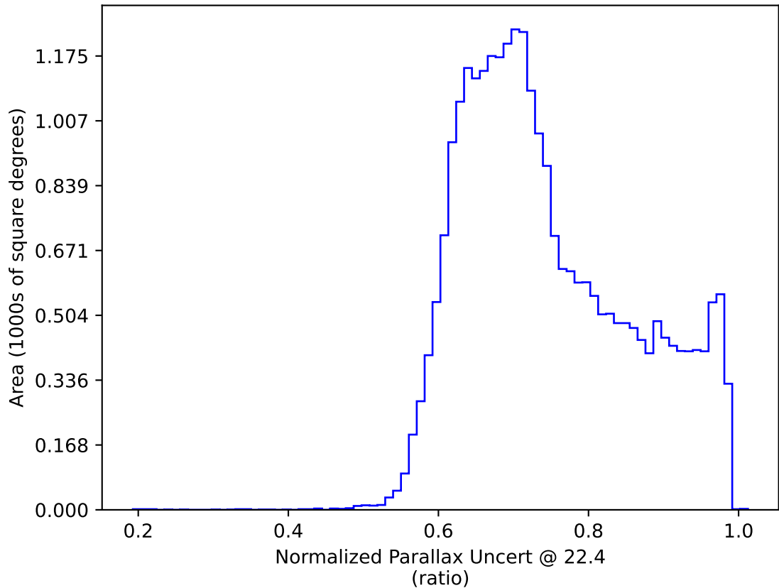
weather_cloudso6v3.4_10yrs All sky: Normalized Parallax Uncert @ 22.4
