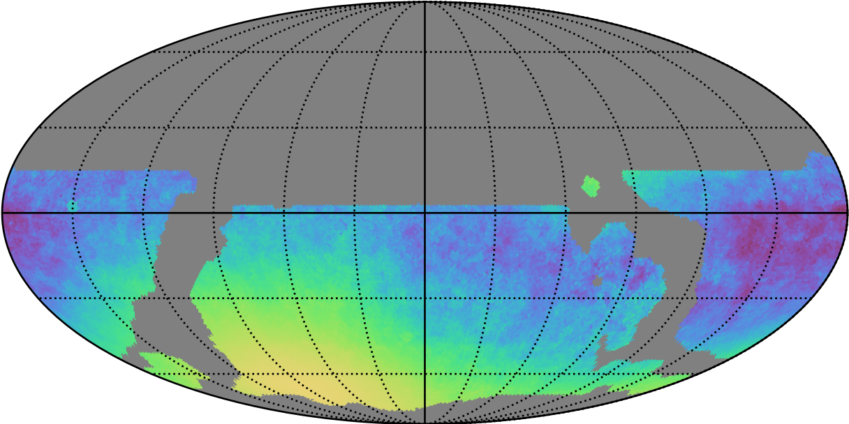
weather_cloudso6v3.4_10yrs WFD y band only: Normalized Parallax Uncert @ 21.3
