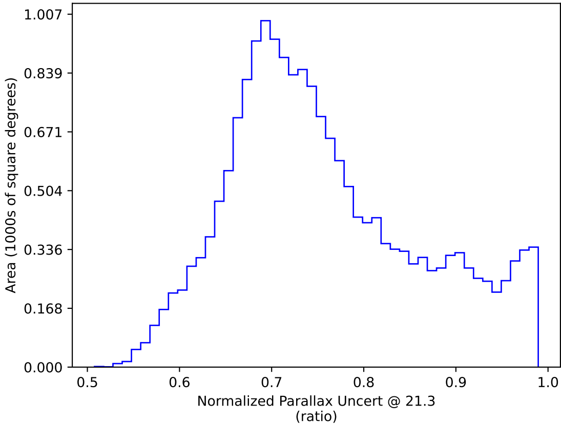
weather_cloudso6v3.4_10yrs WFD y band only: Normalized Parallax Uncert @ 21.3
