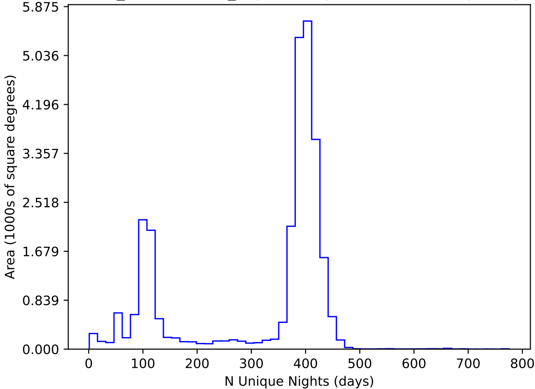
weather_cloudso6v3.4_10yrs All sky all bands: N Unique Nights
