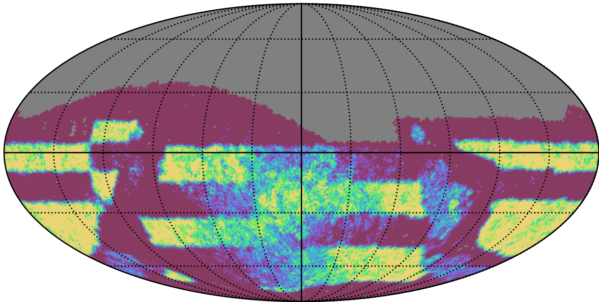
weather_cloudso6v3.4_10yrs Yr 3-4 z band: NVisits
