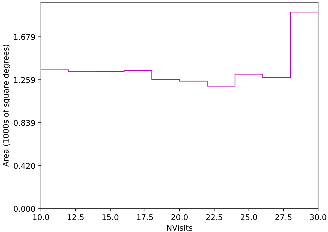
weather_cloudso6v3.4_10yrs Yr 3-4 z band: NVisits
