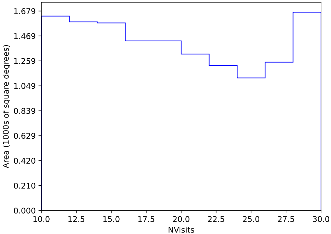
weather_cloudso6v3.4_10yrs Yr 3-4 y band: NVisits
