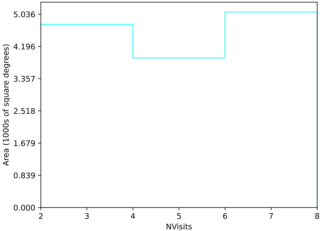
weather_cloudso6v3.4_10yrs Yr 3-4 u band: NVisits
