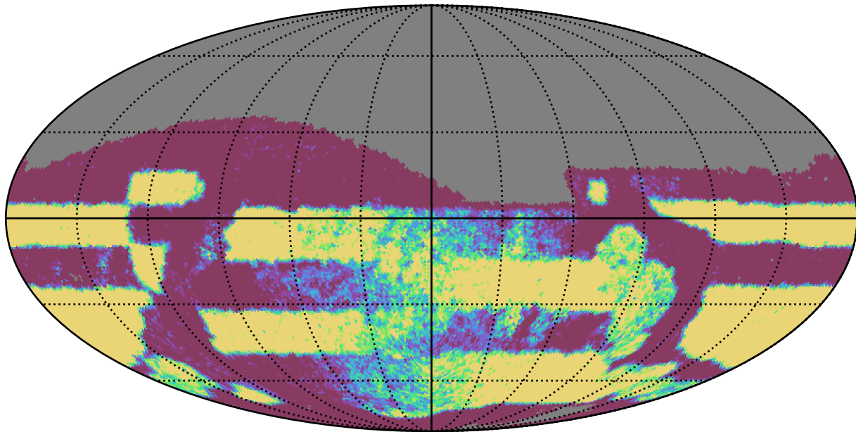
weather_cloudso6v3.4_10yrs Yr 3-4 r band: NVisits
