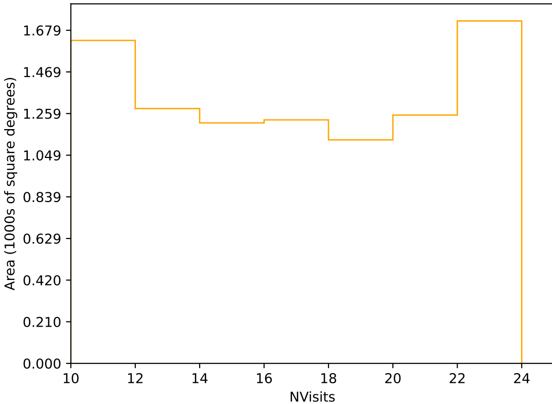
weather_cloudso6v3.4_10yrs Yr 3-4 r band: NVisits
