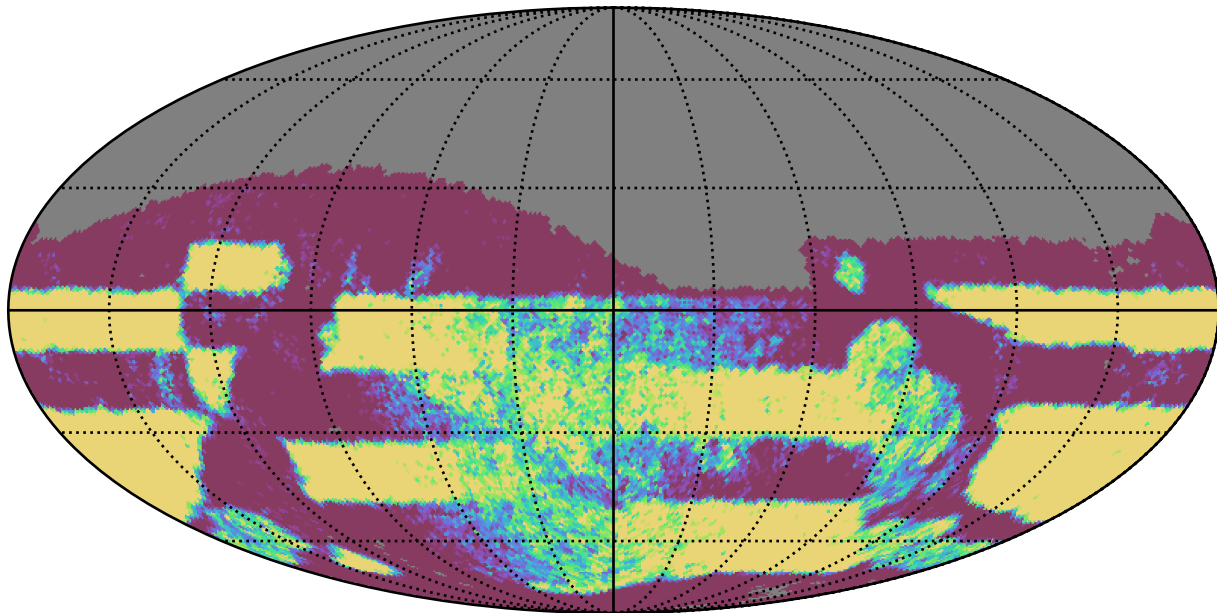
weather_cloudso6v3.4_10yrs Yr 3-4 i band: NVisits
