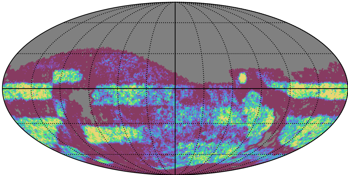
weather_cloudso6v3.4_10yrs Yr 3-4 g band: NVisits
