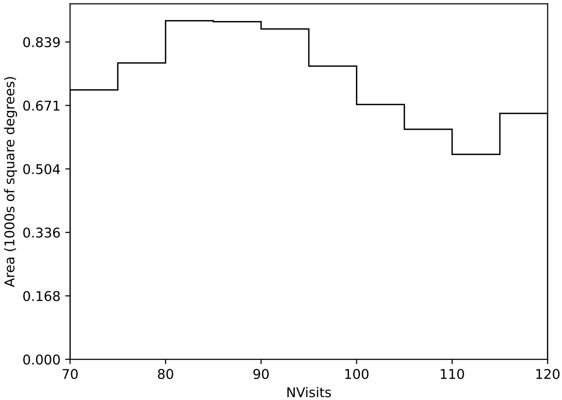
weather_cloudso6v3.4_10yrs Yr 3-4 all bands: NVisits
