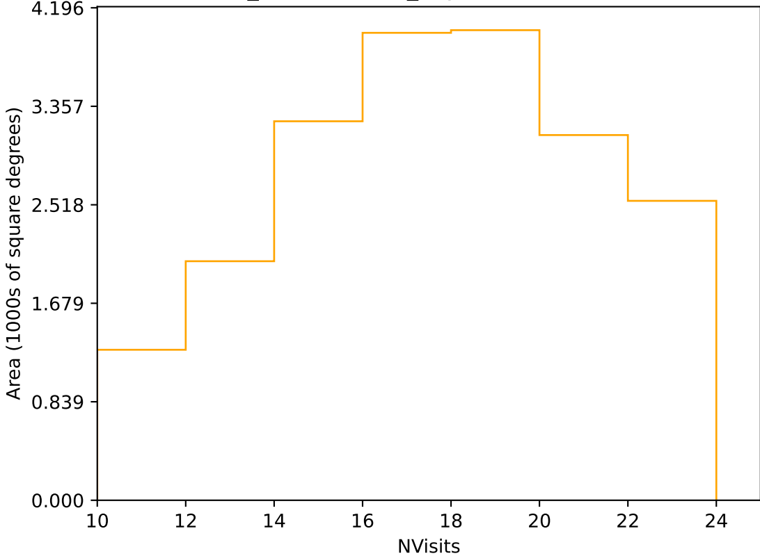
weather_cloudso6v3.4_10yrs Yr 1 r band: NVisits
