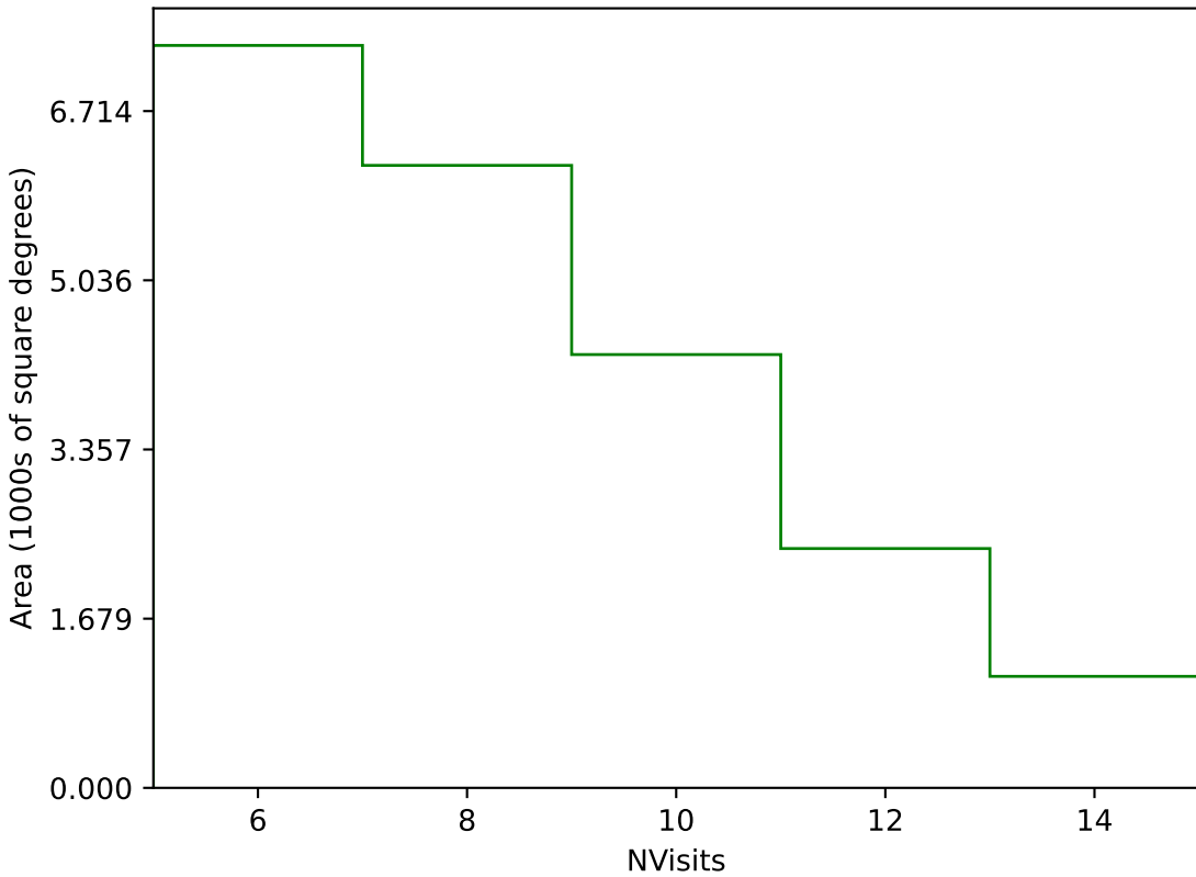
weather_cloudso6v3.4_10yrs Yr 1 g band: NVisits
