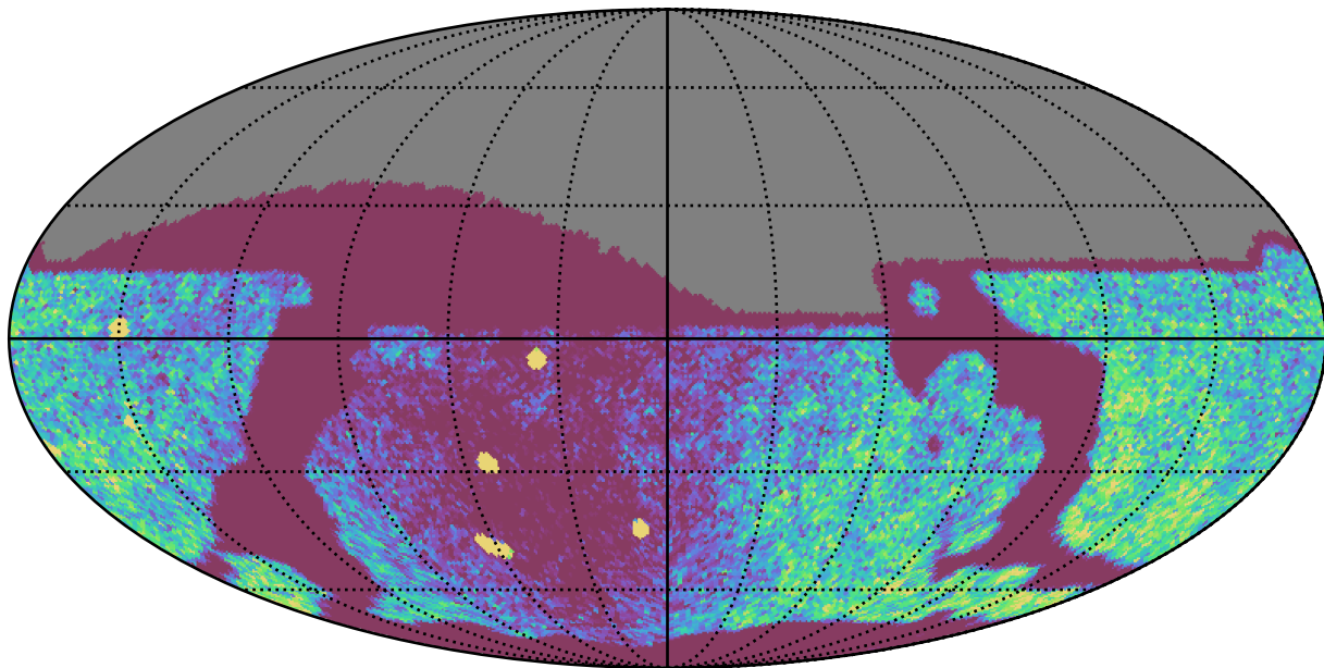
weather_cloudso6v3.4_10yrs Yr 1 all bands: NVisits
