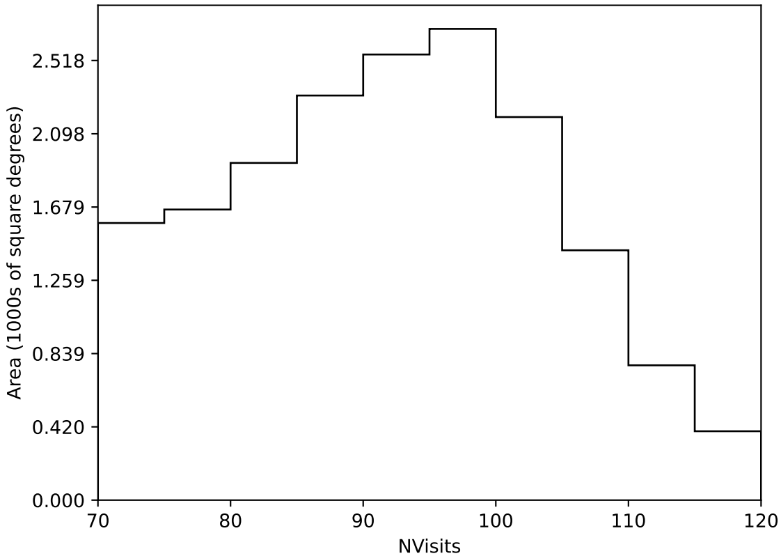
weather_cloudso6v3.4_10yrs Yr 1 all bands: NVisits
