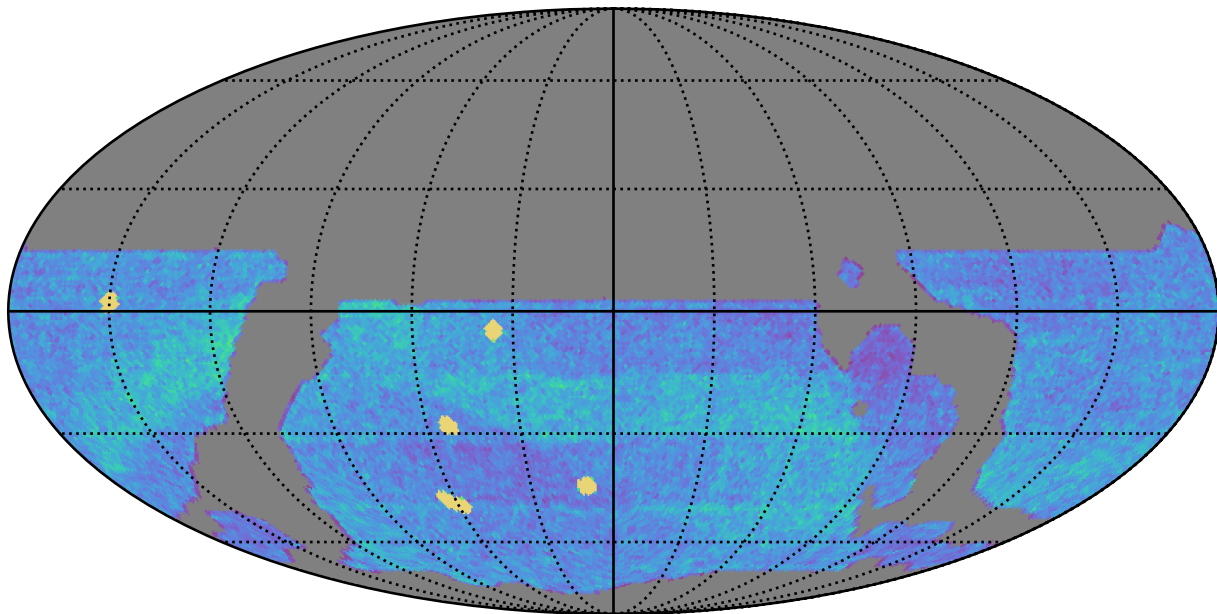
weather_cloudso6v3.4_10yrs WFD all bands: NVisits
