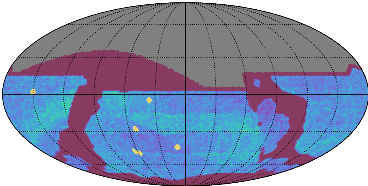
weather_cloudso6v3.4_10yrs All sky all bands: NVisits
