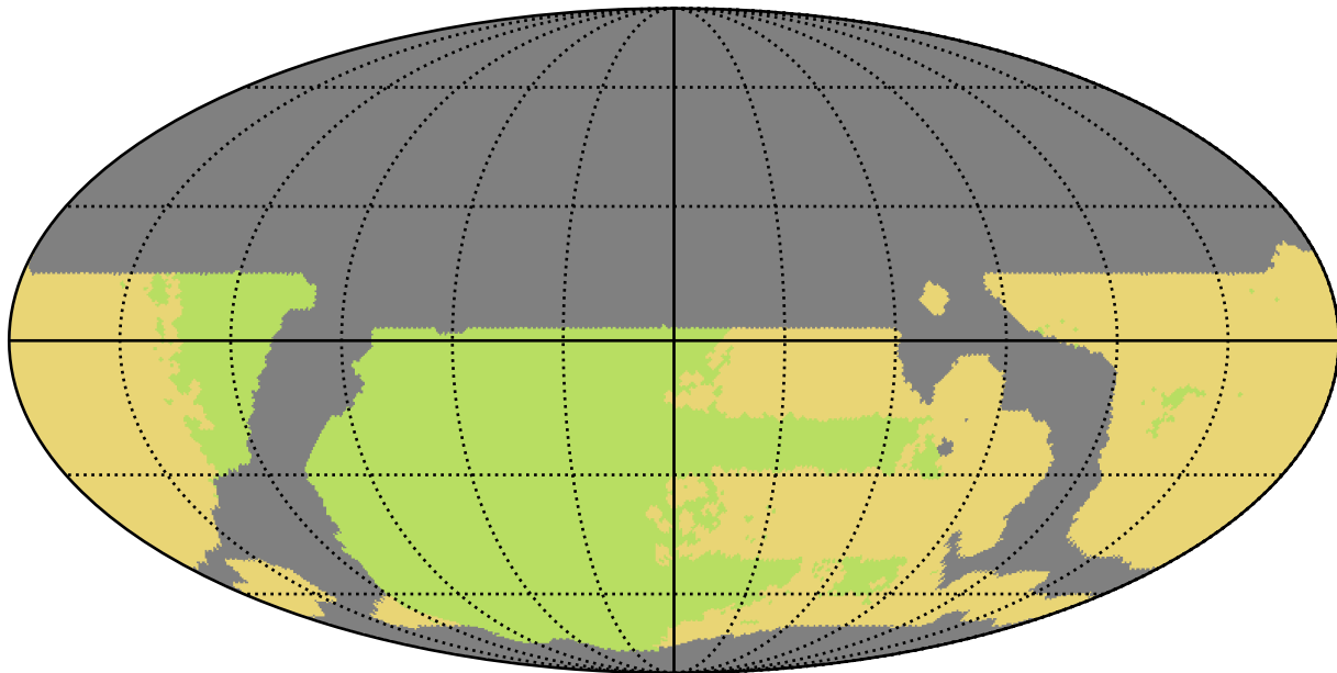
weather_cloudso6v3.4_10yrs WFD all bands: NSeasons
