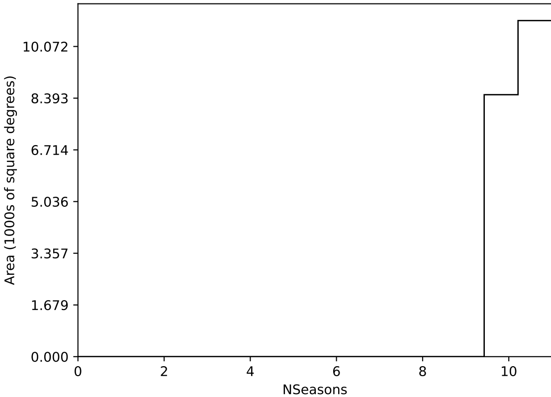
weather_cloudso6v3.4_10yrs WFD all bands: NSeasons
