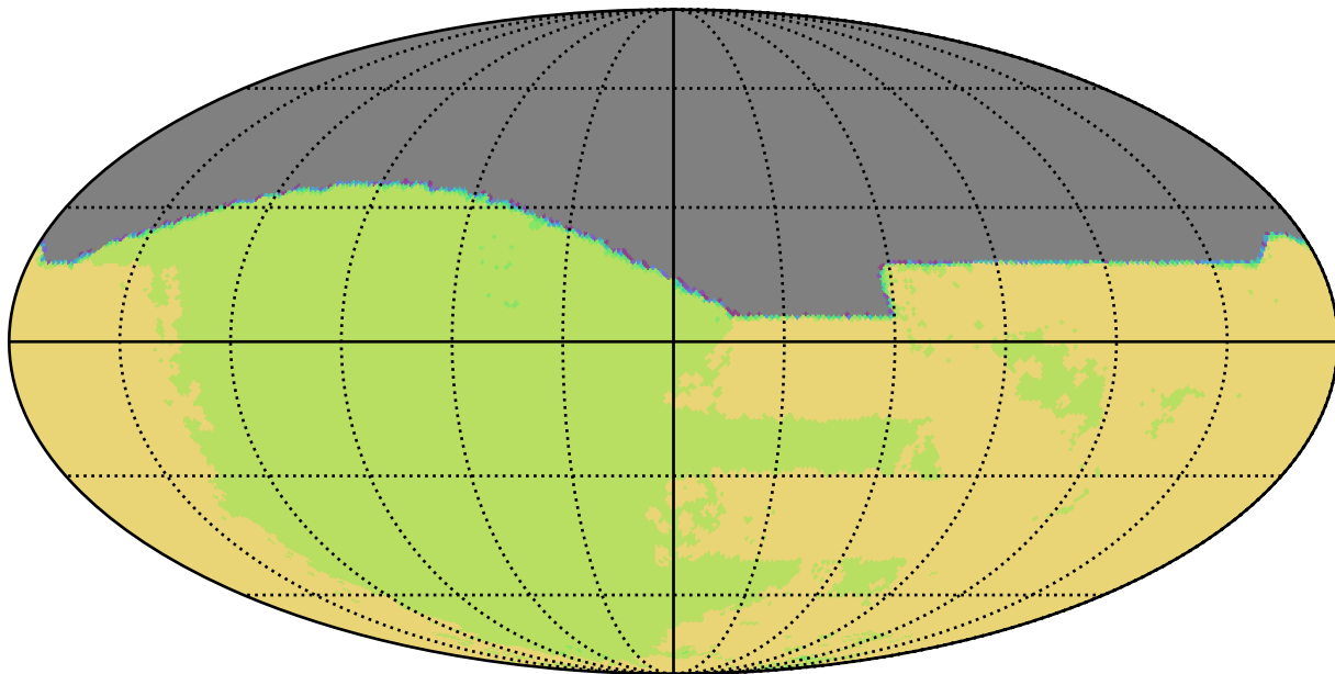
weather_cloudso6v3.4_10yrs All sky all bands: NSeasons
