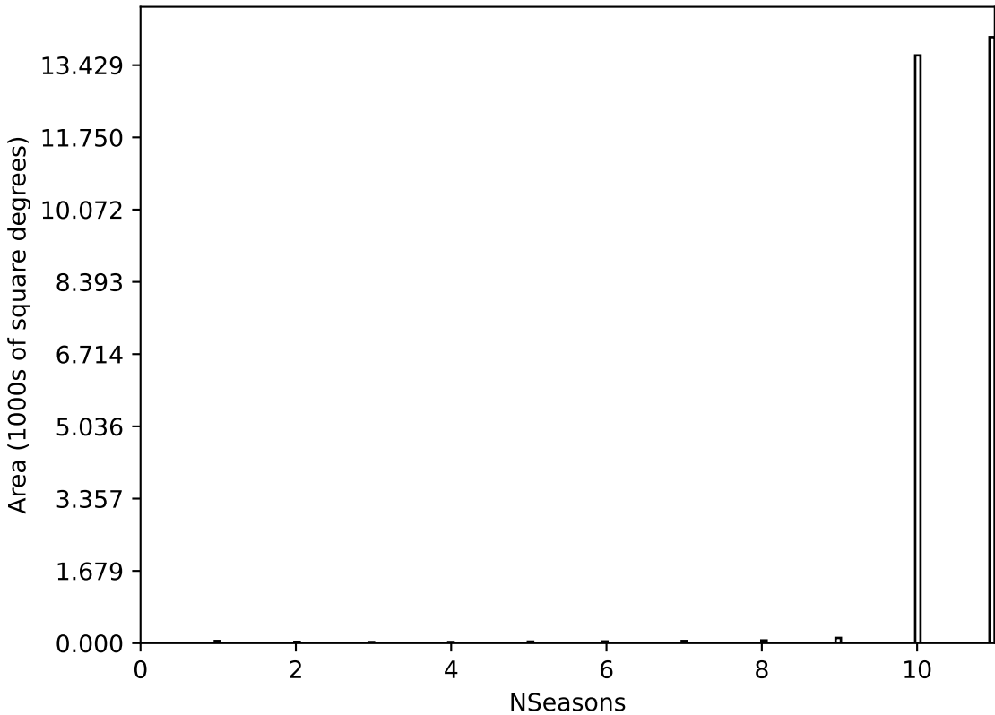
weather_cloudso6v3.4_10yrs All sky all bands: NSeasons
