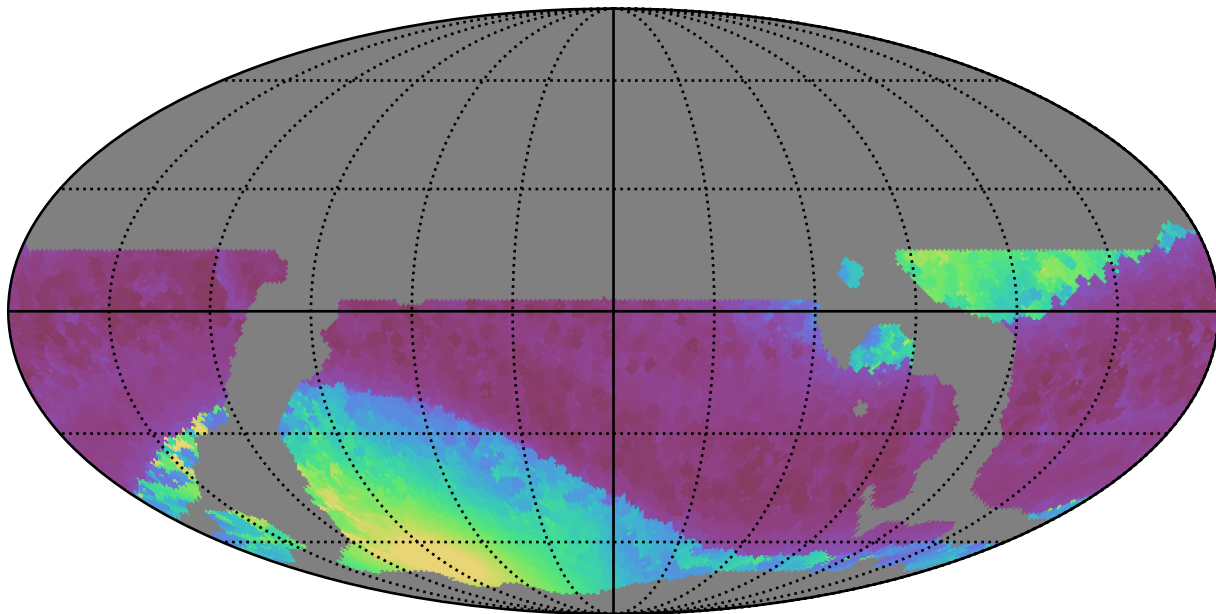
weather_cloudso6v3.4_10yrs WFD all bands: Min solarElong
