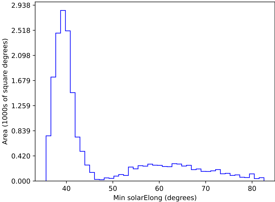
weather_cloudso6v3.4_10yrs WFD all bands: Min solarElong
