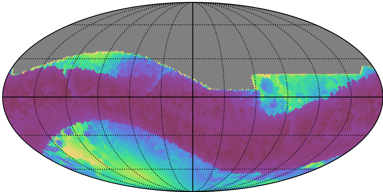
weather_cloudso6v3.4_10yrs All sky all bands: Min solarElong
