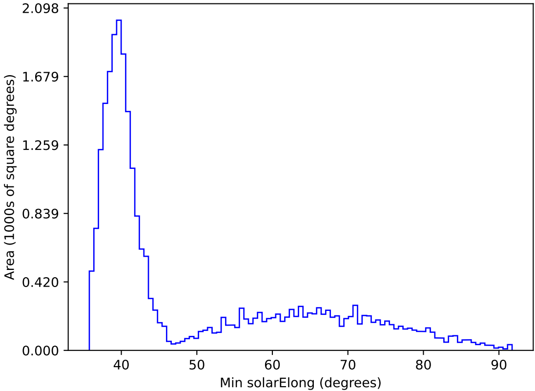
weather_cloudso6v3.4_10yrs All sky all bands: Min solarElong
