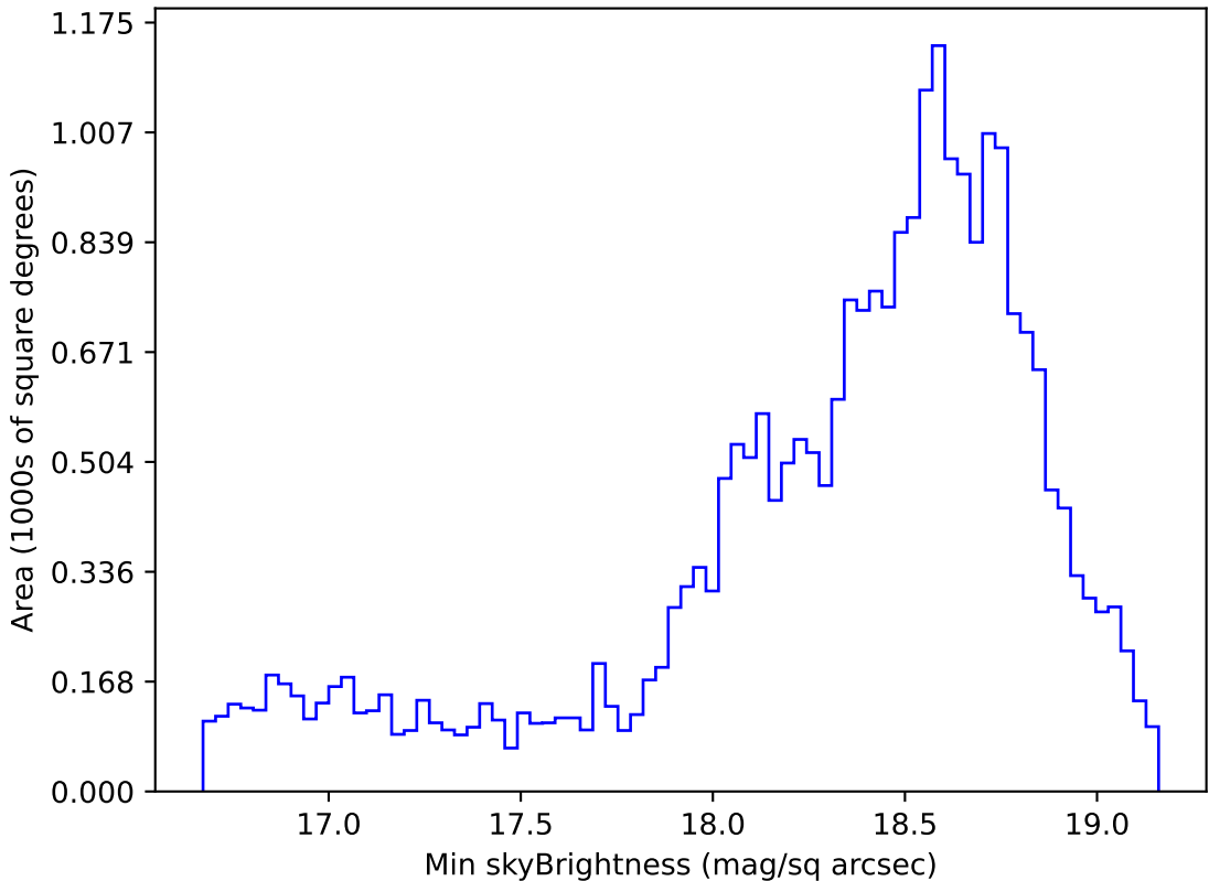
weather_cloudso6v3.4_10yrs Yr 1 z band: Min skyBrightness
